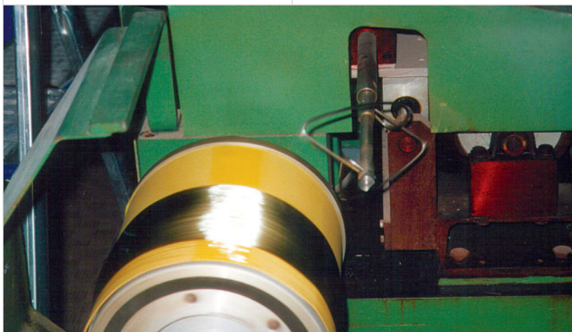
Fly ash being spun into glass fibers.
